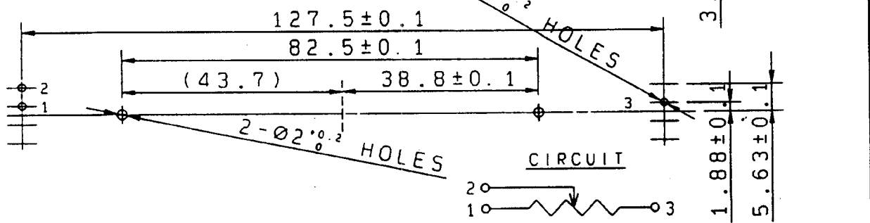
MOUNTING HOLE DETAIL (取付穴寸法図) VIEWED FROM MOUNTING SIDE (挿入側より)
