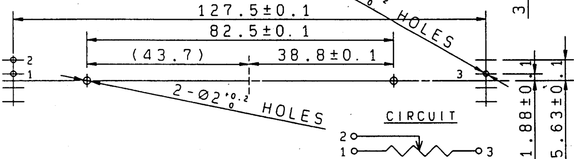
MOUNTING HOLE DETAIL (取付穴寸法図) VIEWED FROM MOUNTING SIDE (挿入側より)
