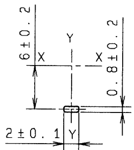
シャフト止め 詳細図 LOCATING LUG DETAIL 軸受取付面 BUSHING MOUNTING SURFACE
