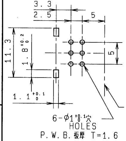
端子取付穴寸法図 (挿入側より見た図) (許容差 ± 0.1) MOUNTING HOLE DETAIL (TOLERANCE ± 0.1) VIEWED FROM MOUNTING SIDE
